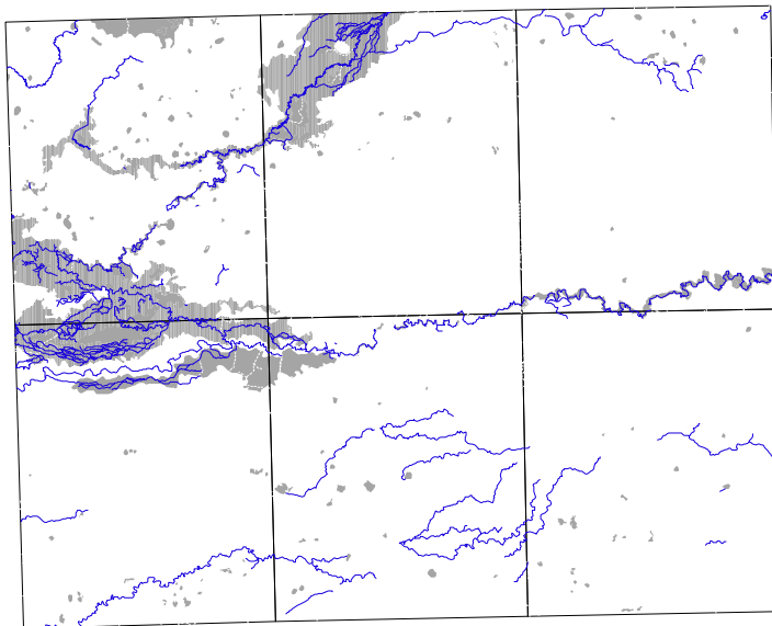
Figure App 5.7 Distribution of quadrat locations for floristic group 19.
