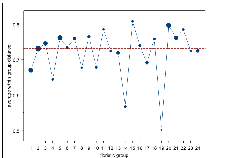
Figure App 5.5 Weighted mean within-group distances for the 24 floristic groups from MRPP (McCune & Mefford 1999).
