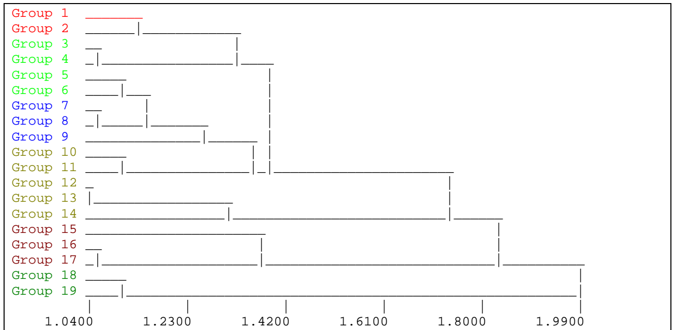
Figure App 5.3 Dendrogram displaying the dissimilarity relationship for a hierarchical analysis.
