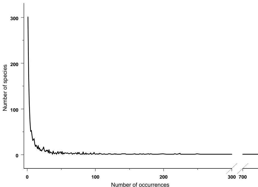
Figure App 5.1 Frequency of occurrence of species in a dataset consisting of 1292 quadrats and 1495 species.
