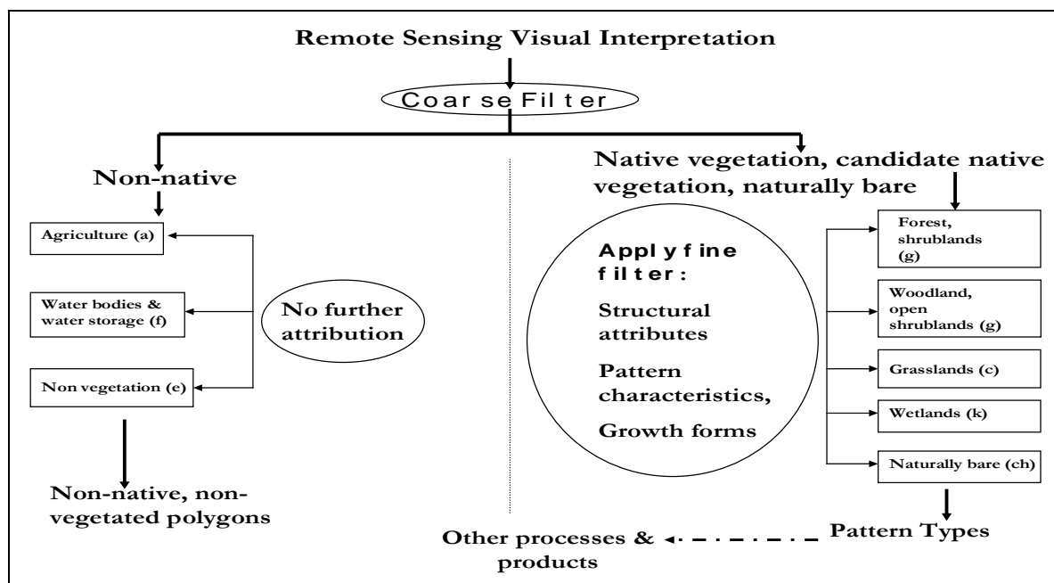
Figure App 2.1 Flow chart showing the level of attribution required for polygons with native and non-native characteristics.
