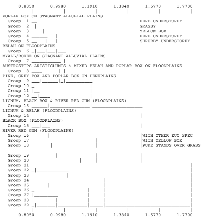
Figure App 5.6 Annotated dendrogram (for comparison with the intuitive classification and interpretation of analysis results).
