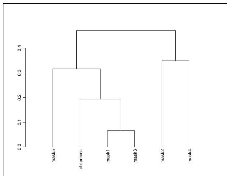
Figure App 5.2 Dendrogram displaying the relationships amongst several data masking options.
